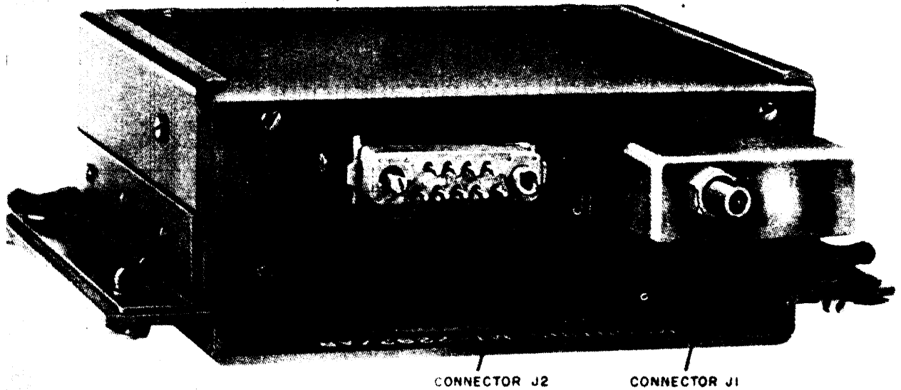
Figure 3. Receiver, Radio R-1041A/ARN attached to Mounting MT-2292/AR, rear view.
